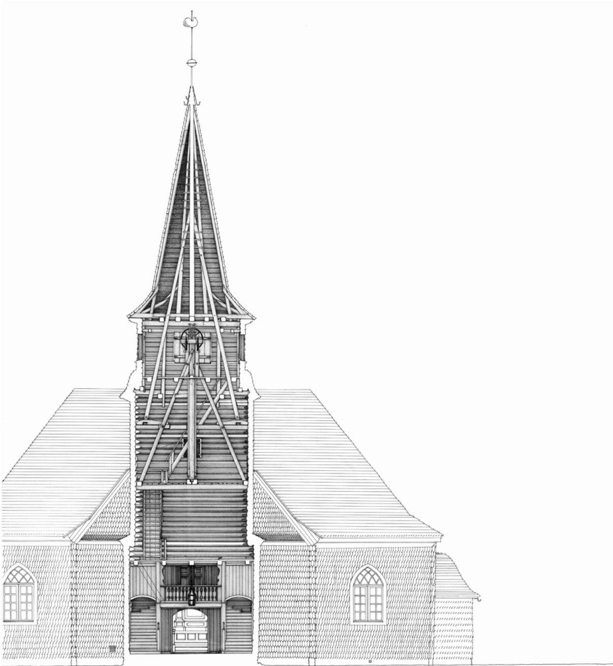
Östmark church, measure drawing by architect professor Sudjit Sananwai
